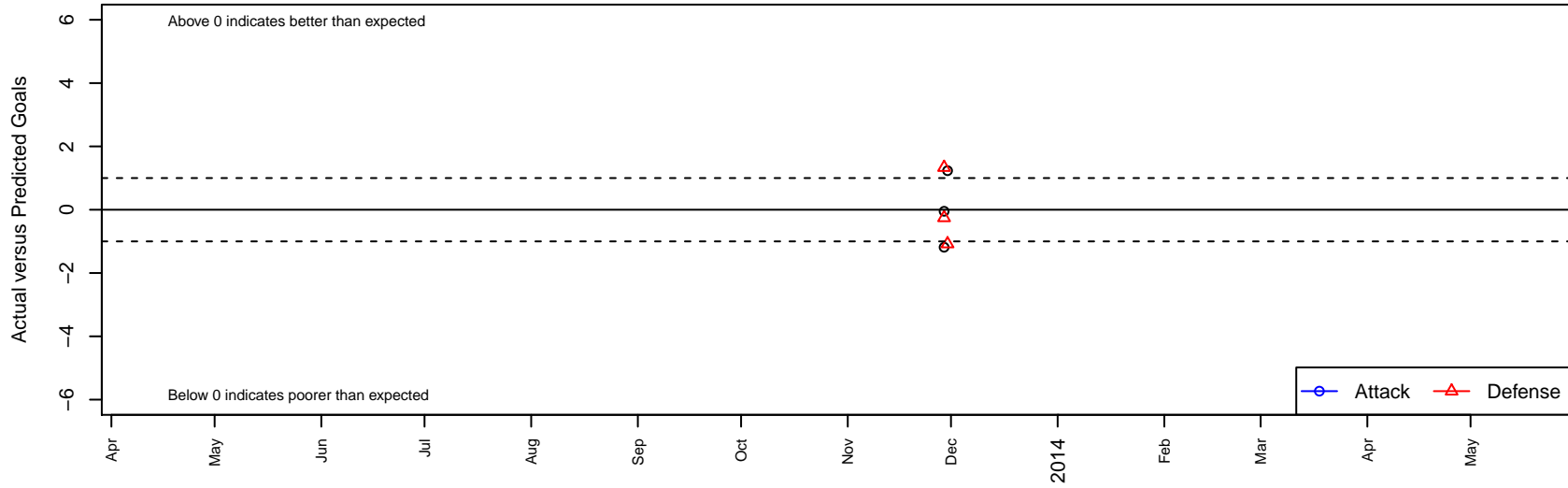
Joga FC 96 B95 Dots are actual minus expected GF (blue circles) and GA (red triangles). Blue line is smoothed change in attack strength. Red is smoothed change in defense strength.
